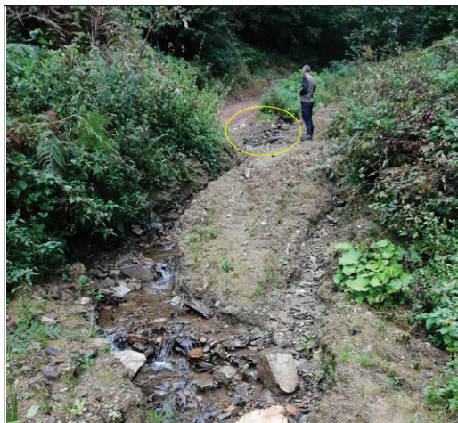
Slika 5. II i IV kategorija uticaja vodotoka na traktorski put i traktorsku vlaklu / Figure 5. II and IV Category of impact of watercourses on skid roads/trails
