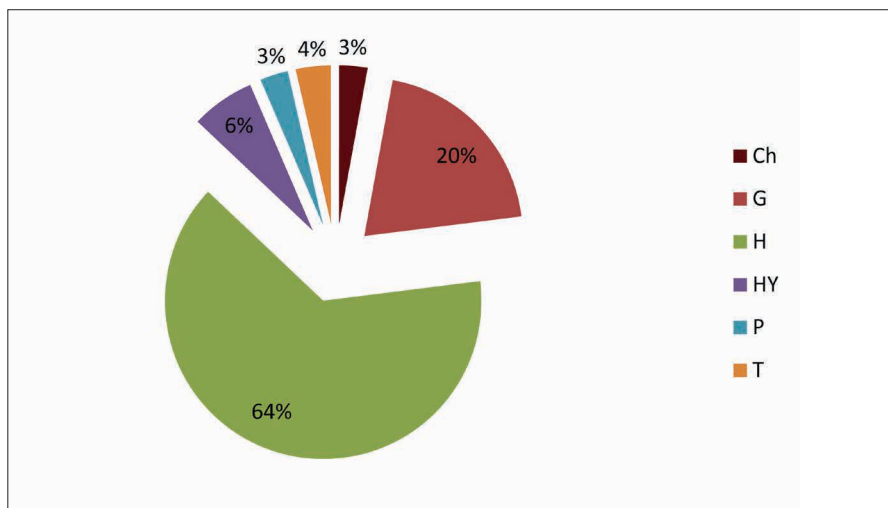
Slika 3. Zastupljenost pojedinih životnih formi u vaskularnoj flori okoline glacijalnih jezera u NP Sutjeska (Ch - hamefite, G - geofite, H - hemikriptofite, HY - hidrofite, P - fanerofite, T - terofite) / Figure 3. Distribution of lifeforms in flora around glacial lakes in Sutjeska NP (Ch - Chamaephytes, G - Geophytes, H - Hemicryptophytes, HY - Hydrophytes, P - Phanerophytes, T - Therophytes)
